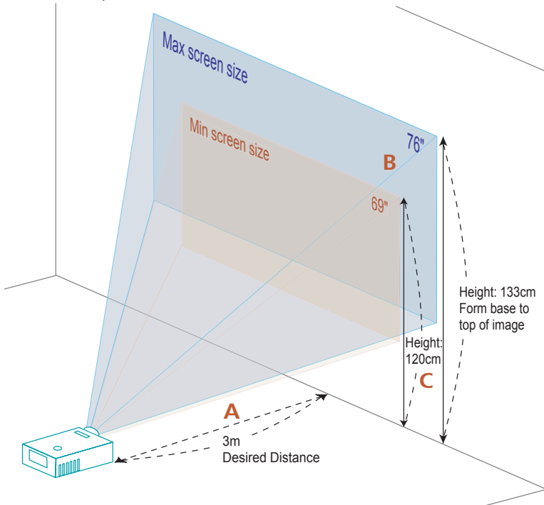
Figure: Fixed distance with different zoom and screen size. (only for X1260 series, X1160 series is Fixed zoom lens)
